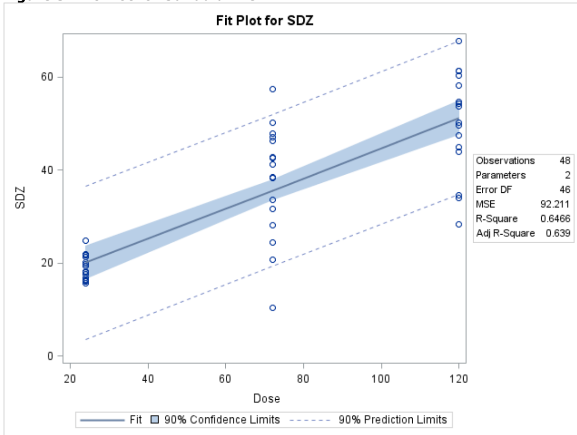
Figure 3. Fit Plot for Sulfadiazine
