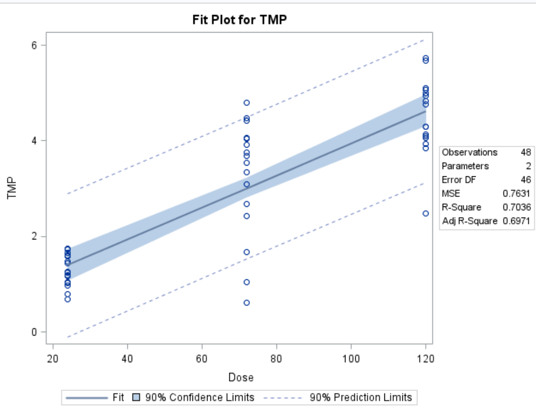
Figure 4. Fit Plot for Trimethoprim
